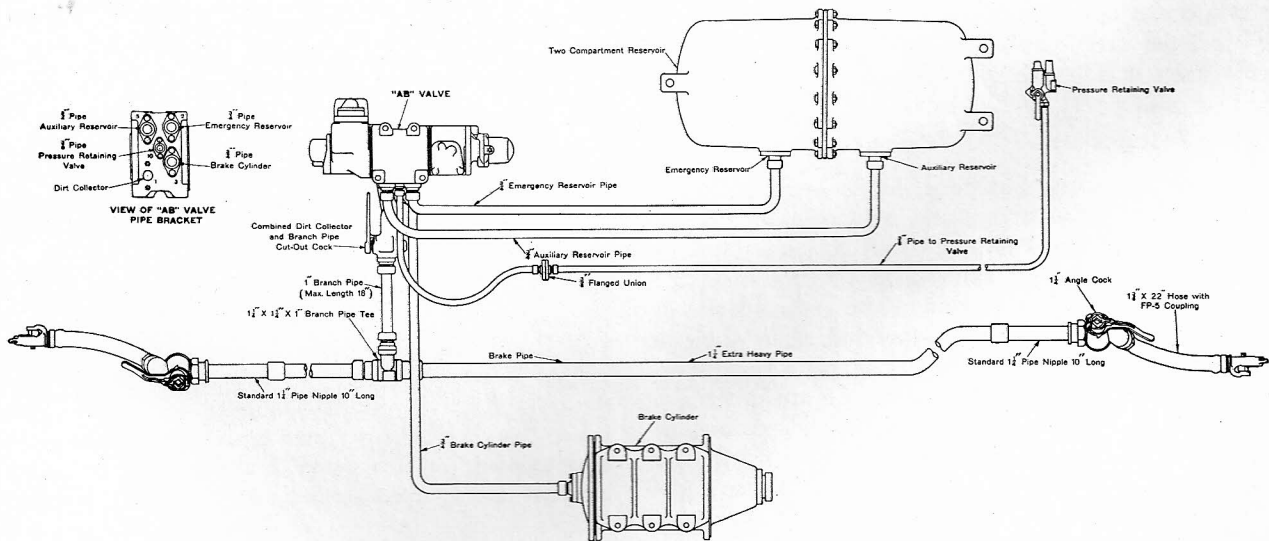
Fig. 2484—Piping diagram of Westinghouse "AB" freight car brake equipment.
