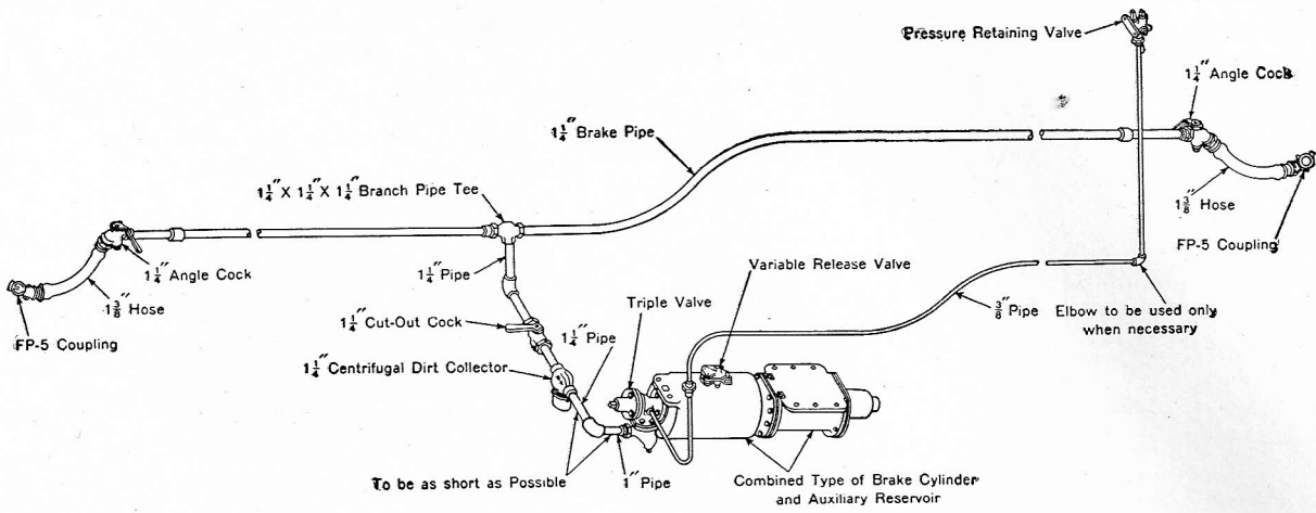
Fig. 2483—Piping diagram of Westinghouse "KC" freight car brake equipment.
