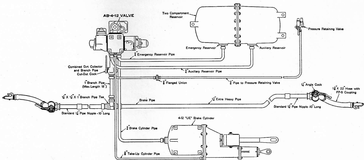
Fig. 2485—Piping diagram of Westinghouse "AB" 4-12 freight brake equipment for very heavy cars.
